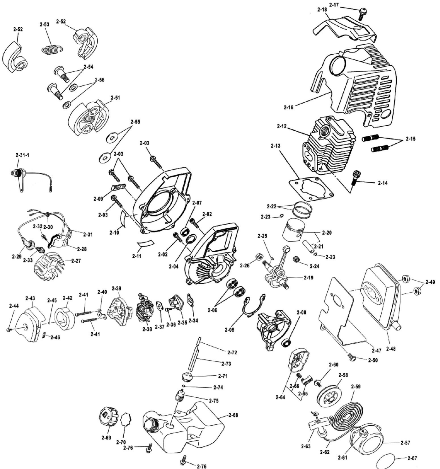
Fig 2. Engine Parts
